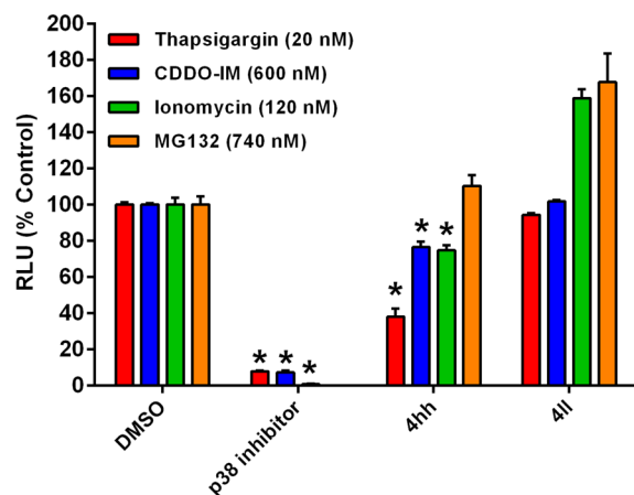
Figure 7. Active benzodiazepinone 4hh , but not inactive compound 4II , inhibits calcium regulator-induced p38 MAPK activation. H4-CHOP-luciferase reporter cells were pretreated with DMSO or compounds for 1 h and then treated with thapsigargin (20 nM), CDDO-IM (600 nM), ionomycin (120 nM), or MG132 (740 nM) for an additional 18 h. The luciferase expression was assessed using the Steady-Glo luciferase assay reagent. The p38 inhibitor was used at 20 \mu M. The benzodiazepinones 4hh or 4II (10 \mu M) were used with thapsigargin or CDDO-IM treatment, while concentrations of 20 and 50 \mu M were tested with MG132 and ionomycin treatment, respectively. Wells treated with compounds only but no inducers were used as background control correspondingly, and wells treated with inducers but no compounds were used as 100% controls. The RLU (% of control) = 100 \times (\text{well value} - \text{average of background}) / (\text{average of 100\% control} - \text{average of background}) . The data were analyzed using MS Excel software. The experiments were repeated at least three times, and the data are represented as the average \pm SEM. Statistical significance ( P < 0.05 ) was determined using one-way analysis of variance. *Significance was compared with inducer treatment groups.
